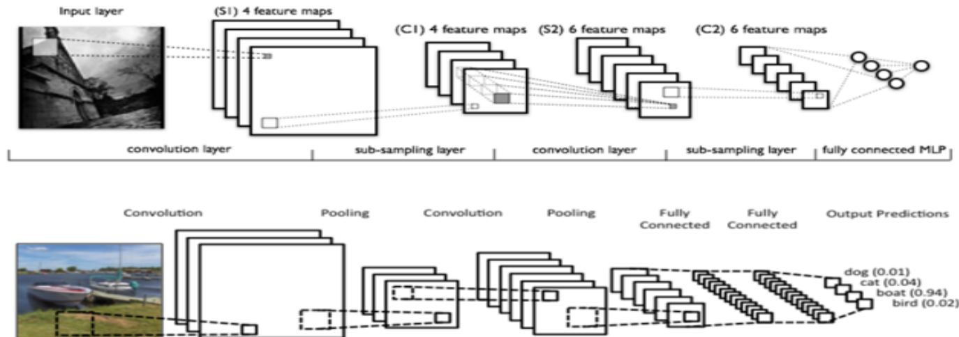
Fig. 5: CNN concept
