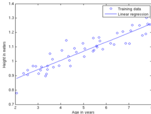
Fig. 3: Linear Regression [17]
