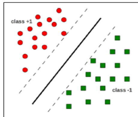
Fig. 2: SVM Algorithm [1]
