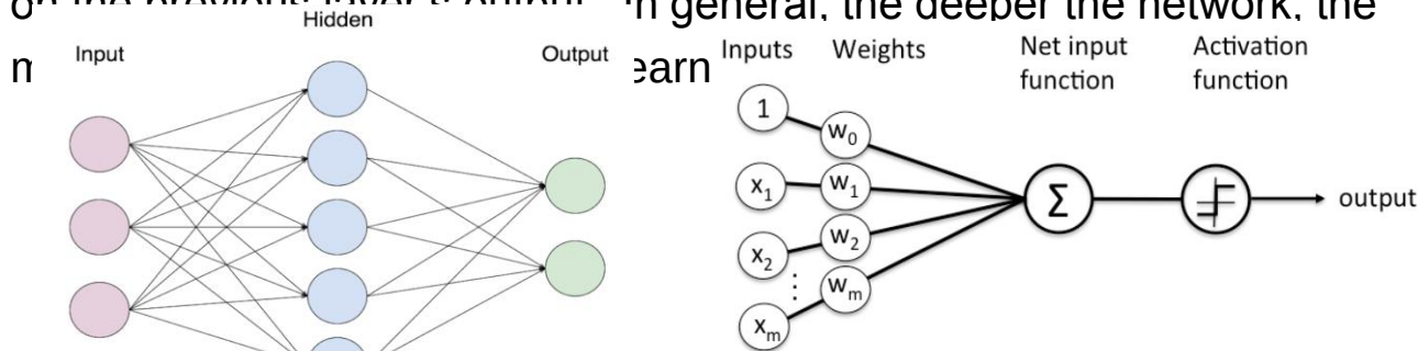
Fig. 4: NN Concept
